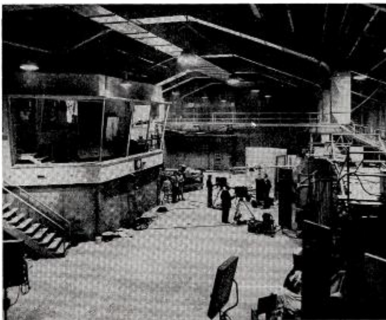
THIS is the principal TV studio of WDSU-AM-FM-TV New Orleans which has just been completed. Dimensions of the studio are 100 x 55 ft., and it is one of four (two AM and one other to be used for AM and TV interchangeably) which are included in the new studio building located directly behind Brulatour Court. Of the approximate $1,200,000 investment by WDSU in radio and TV services, well over one-half million is directly allocated to video, according to the station.
